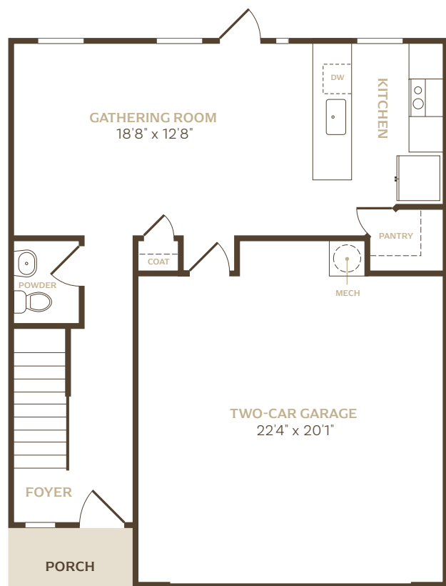
DOWNSTAIRS
